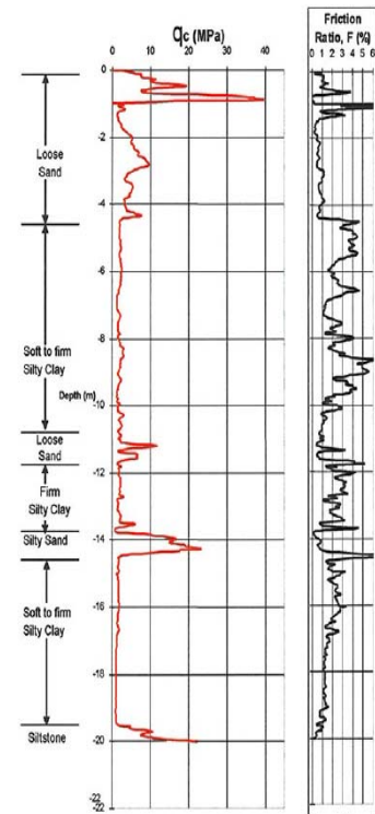
Figure 3: Inferred ground profile and typical CPT data
