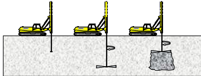
Figure 4: Schematic of jet grouting construction procedure.
